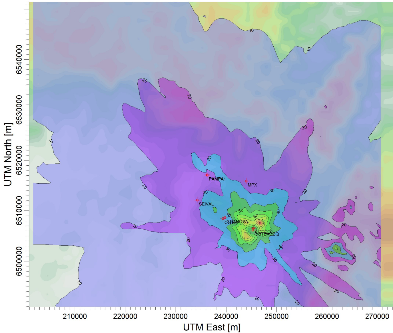
PLOT FILE OF HIGH 1ST HIGH 24-HR VALUES FOR SOURCE GROUP: TODAS Max: 108 [ \mu\text{g}/\text{m}^3 ] at (246749,00; 6507569,00)
