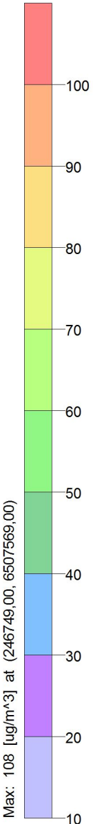
PLOT FILE OF HIGH 1ST HIGH 24-HR VALUES FOR SOURCE GROUP: TODAS Max: 108 [ \mu\text{g}/\text{m}^3 ] at (246749,00; 6507569,00)
