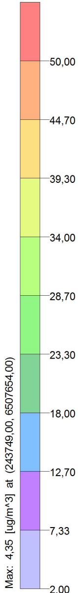
PLOT FILE OF HIGH 1ST HIGH MONTH VALUES FOR SOURCE GROUP: TODAS Max: 4,35 [ \mu\text{g}/\text{m}^3 ] at (243749,00, 6507654,00)
