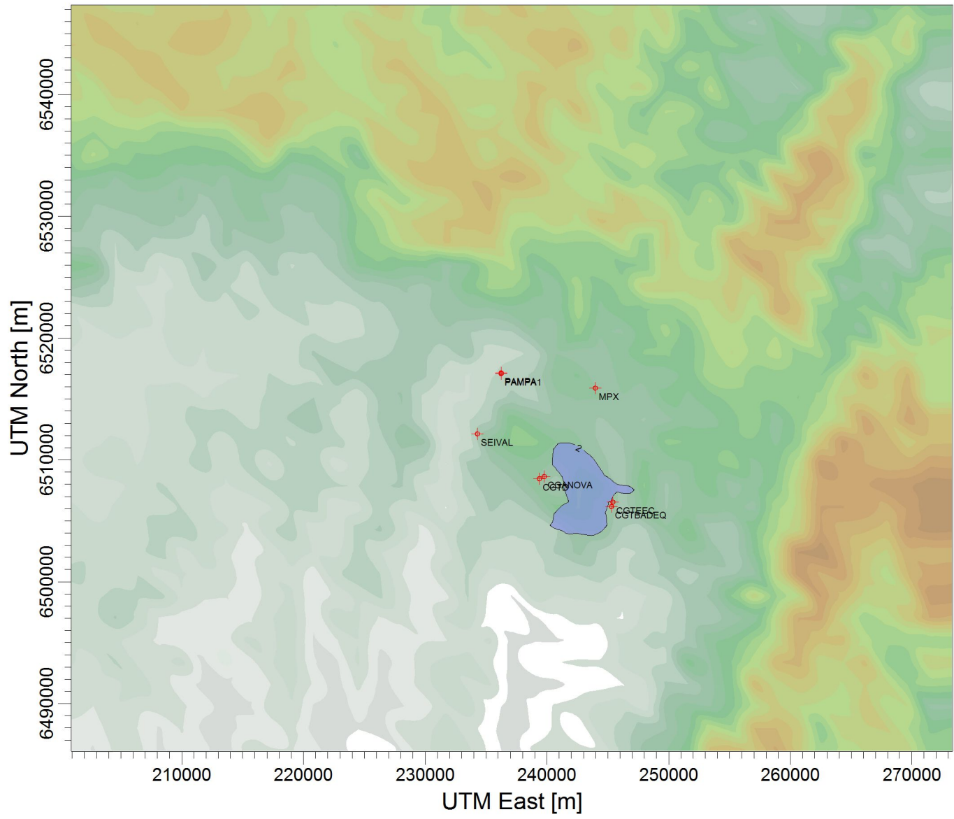
PLOT FILE OF HIGH 1ST HIGH MONTH VALUES FOR SOURCE GROUP: TODAS Max: 4,35 [ \mu\text{g}/\text{m}^3 ] at (243749,00, 6507654,00)
