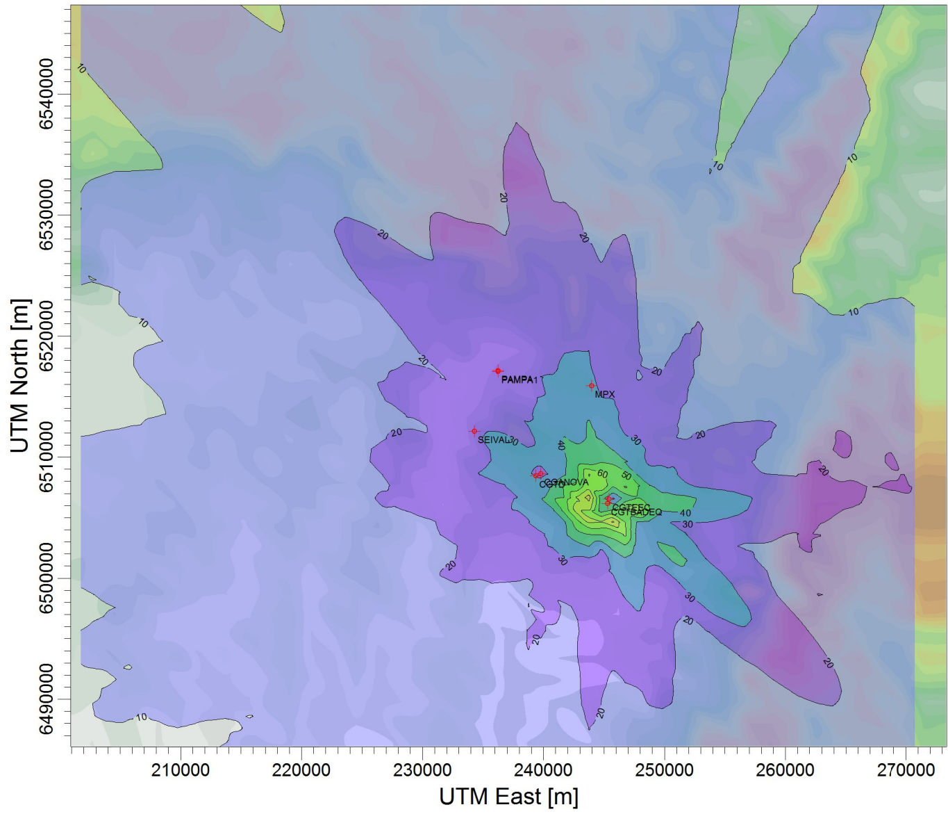
PLOT FILE OF HIGH 1ST HIGH 24-HR VALUES FOR SOURCE GROUP: TODAS Max: 84,9 [\mu\text{g}/\text{m}^3] at (243749,00, 6506654,00)
