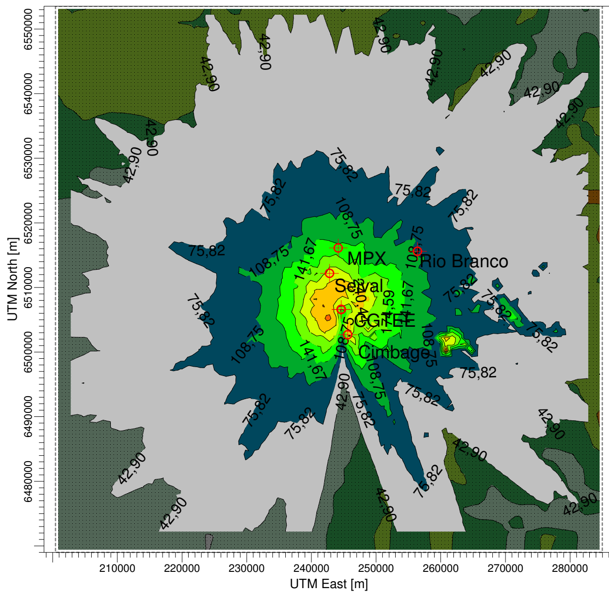
PLOT FILE OF HIGH 1ST HIGH 1-HR VALUES FOR SOURCE GROUP: ATUAL
