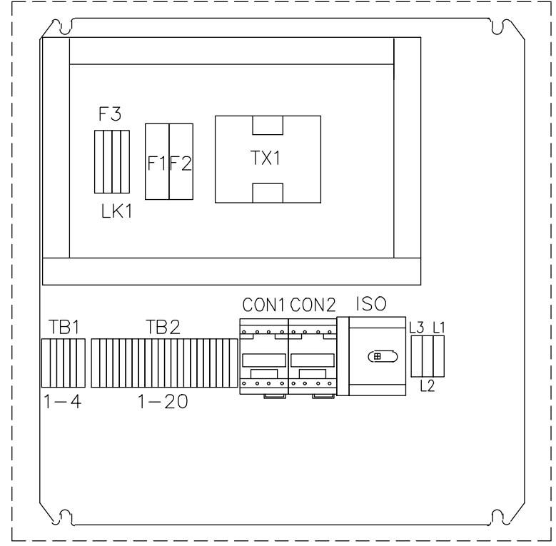
INTERNAL ARRANGEMENT
