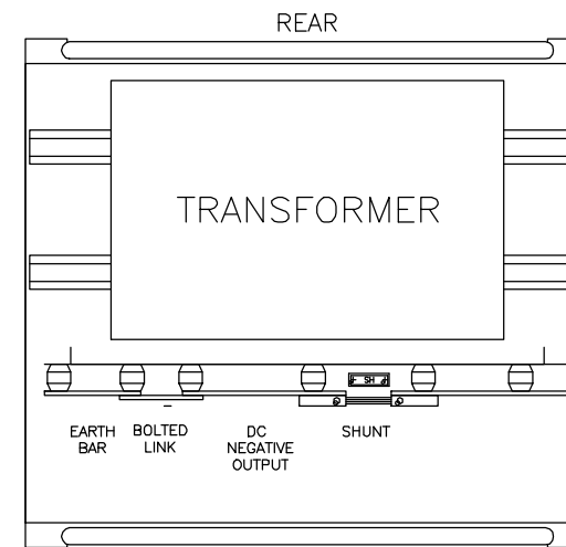
FRONT BASE VIEW
