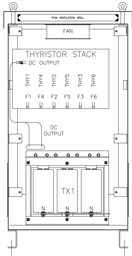
REAR VIEW
