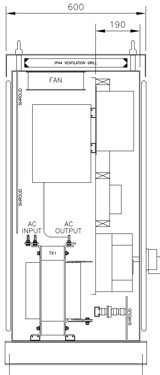
SIDE VIEW
