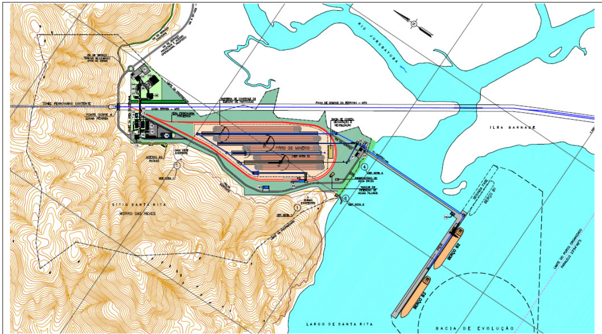
Figura 2.2-2: Layout do Terminal Brites
