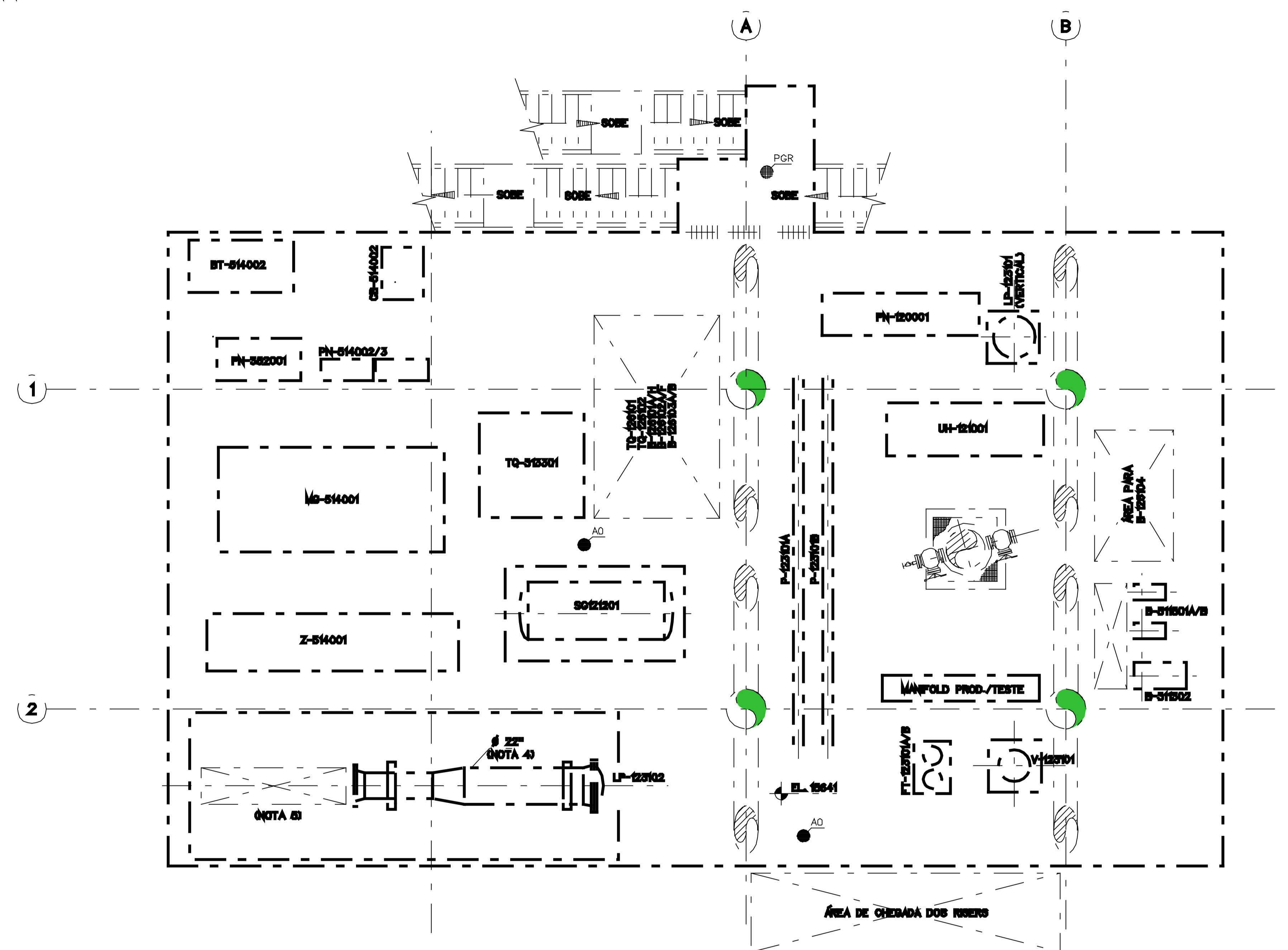
CONVÉS INFERIOR EL. 15641
