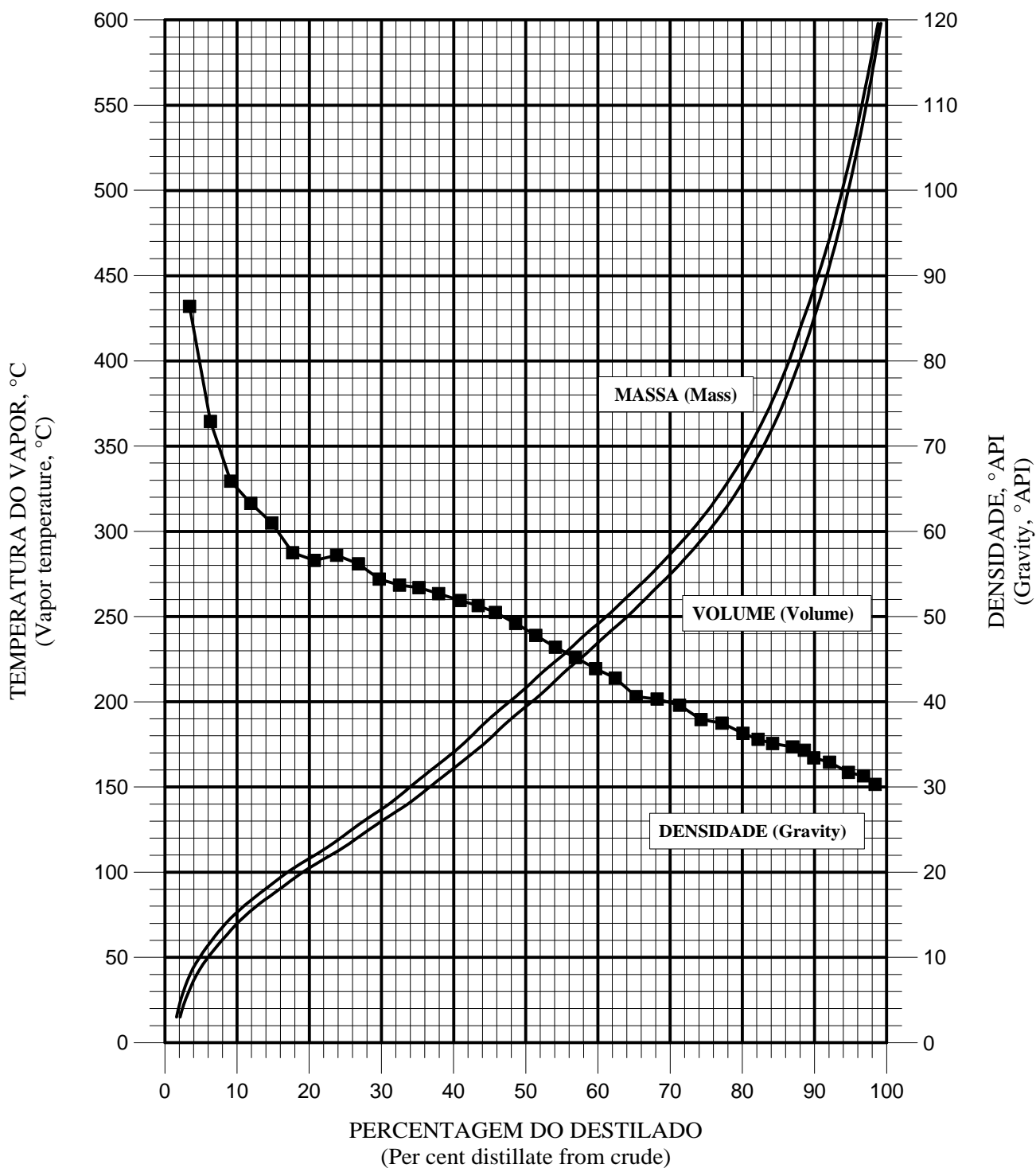
Fig. 1 - Petróleo 3-SPS-41D-TFR-01 - 48,3 °API. Curvas PEV - °API versus ponto médio volumétrico. (TBP curves - Gravity, °API of cuts versus middle volume per cent).
