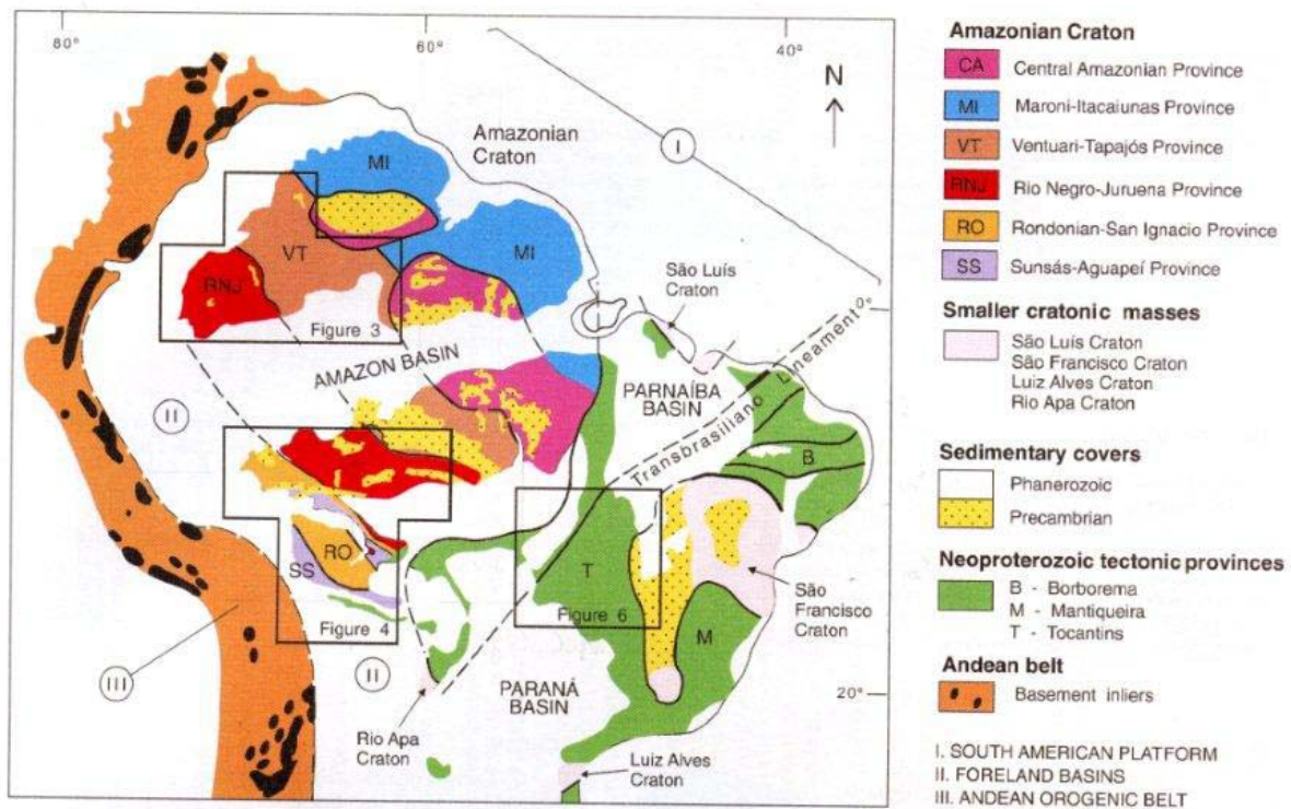
Proterozoic accretionary belts in the Amazonian Craton
