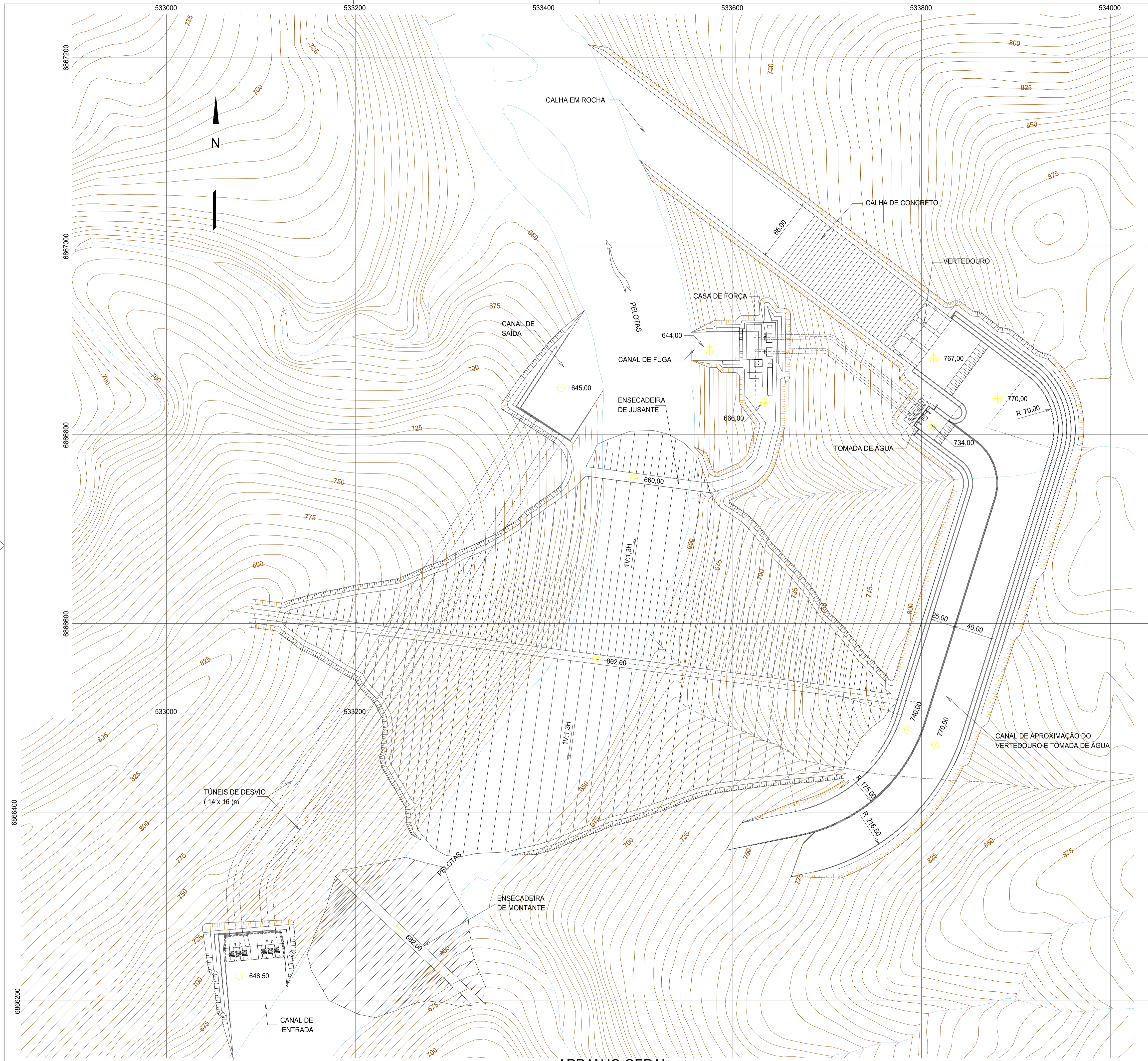
ARRANJO GERAL
