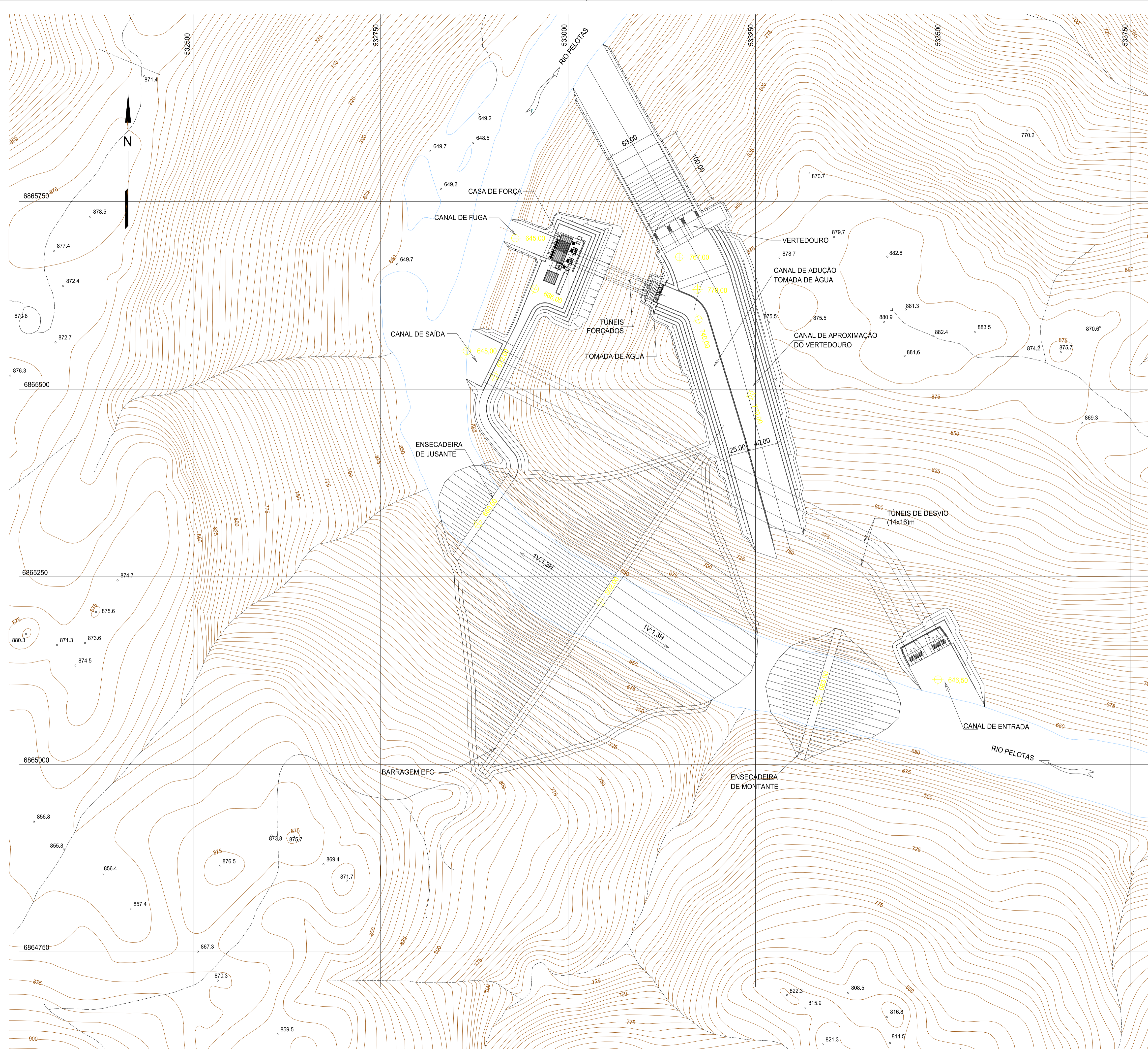
ARRANJO GERAL
