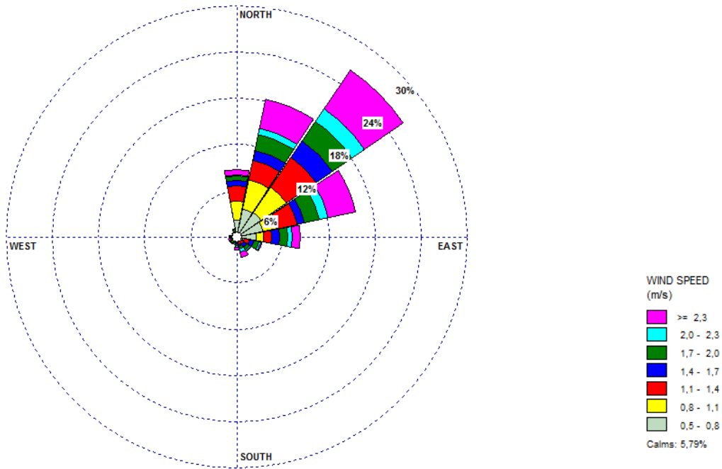
Wind Class Frequency Distribution
