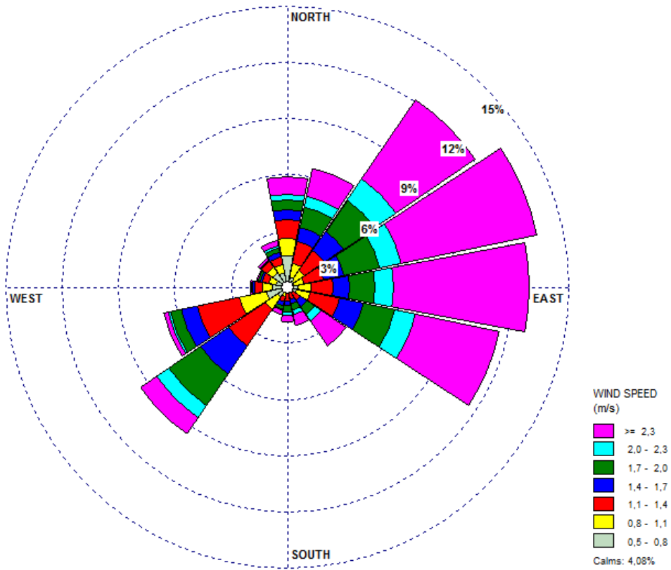
Wind Class Frequency Distribution
