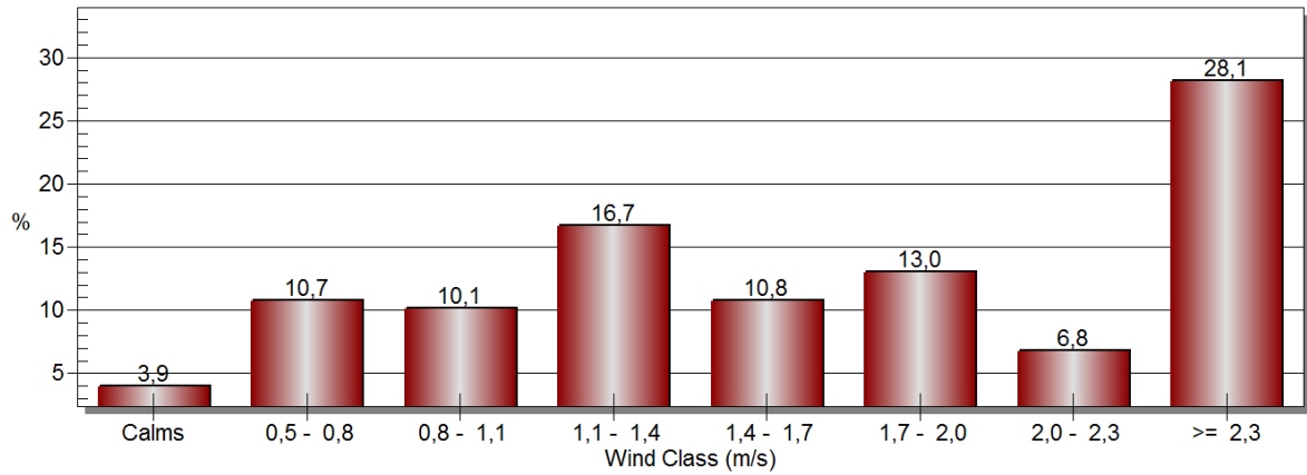
Wind Class Frequency Distribution
