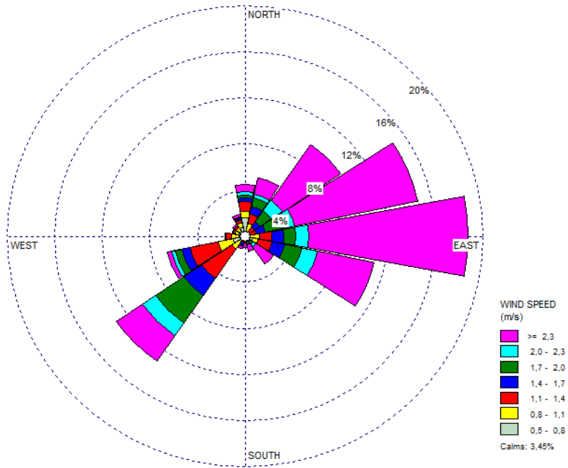
Wind Class Frequency Distribution
