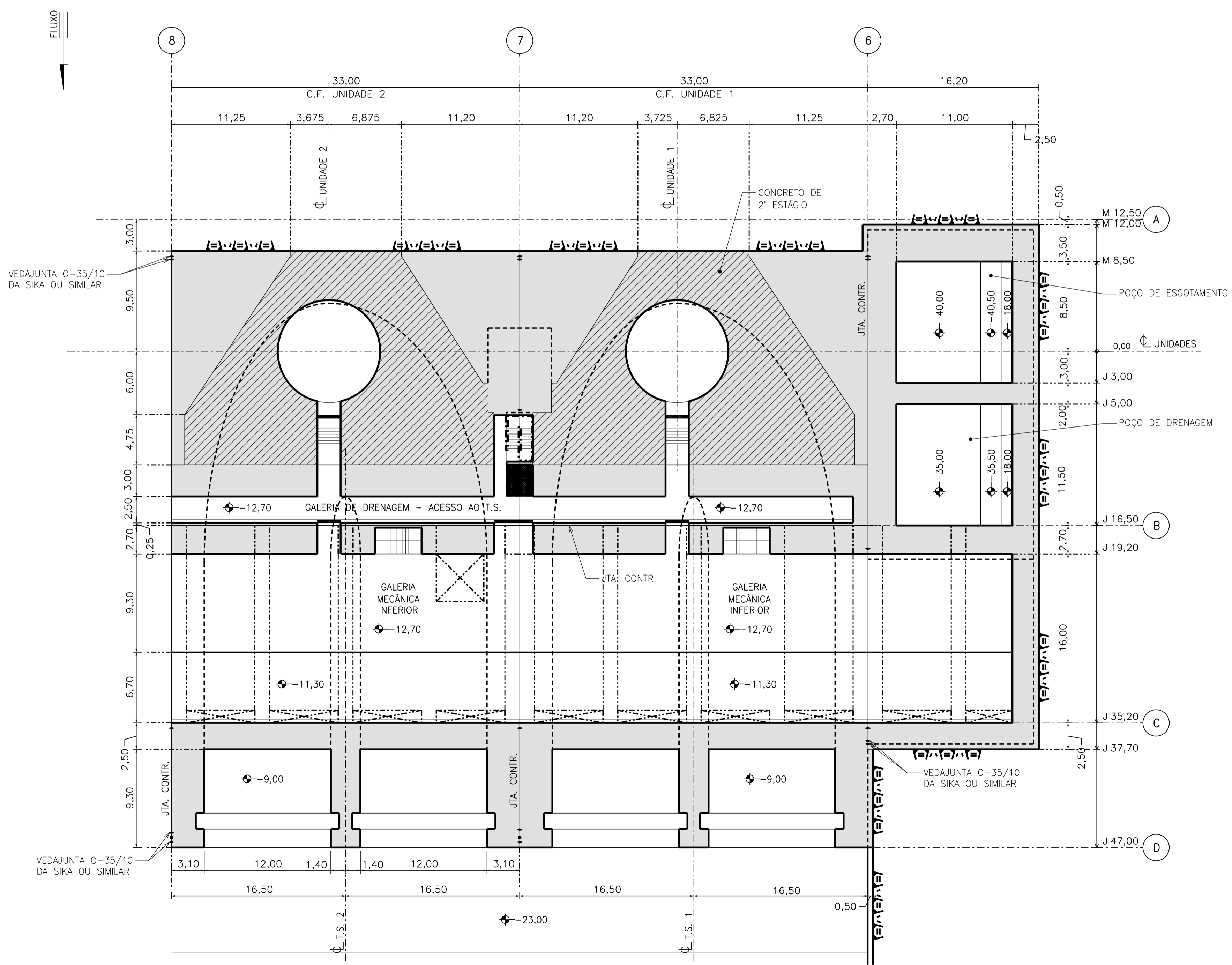
PLANTA EL. -9,50
