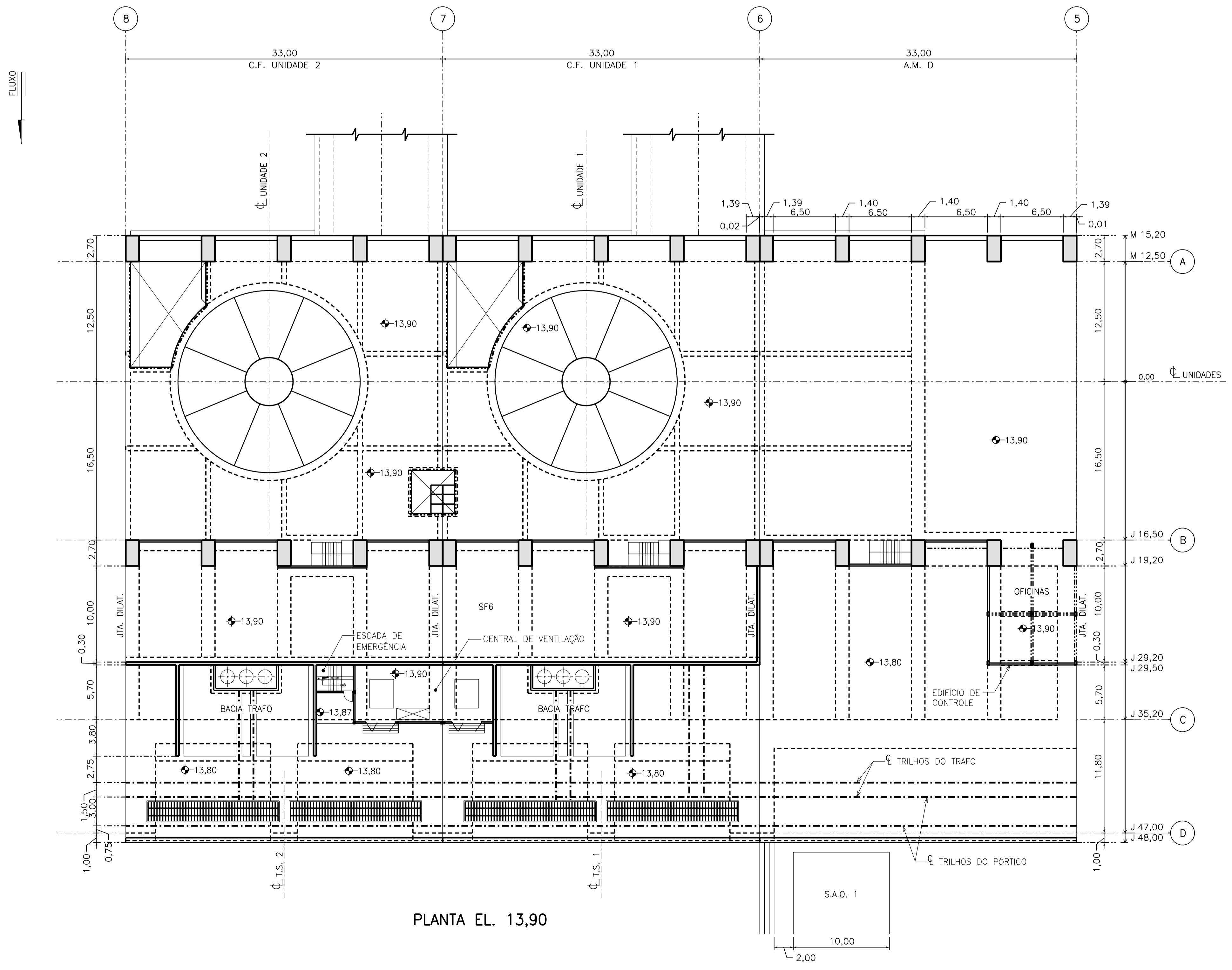
PLANTA GERAL ORIENTATIVA EL. 13,90
