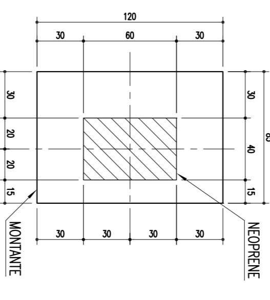
MONTANTES: 85/120/21.5 (4x) ESCALA = 1/25
